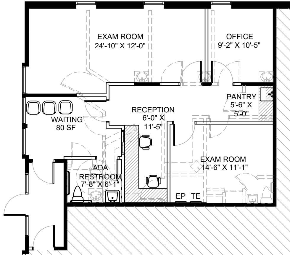
Proposed Space Plan- First Floor
