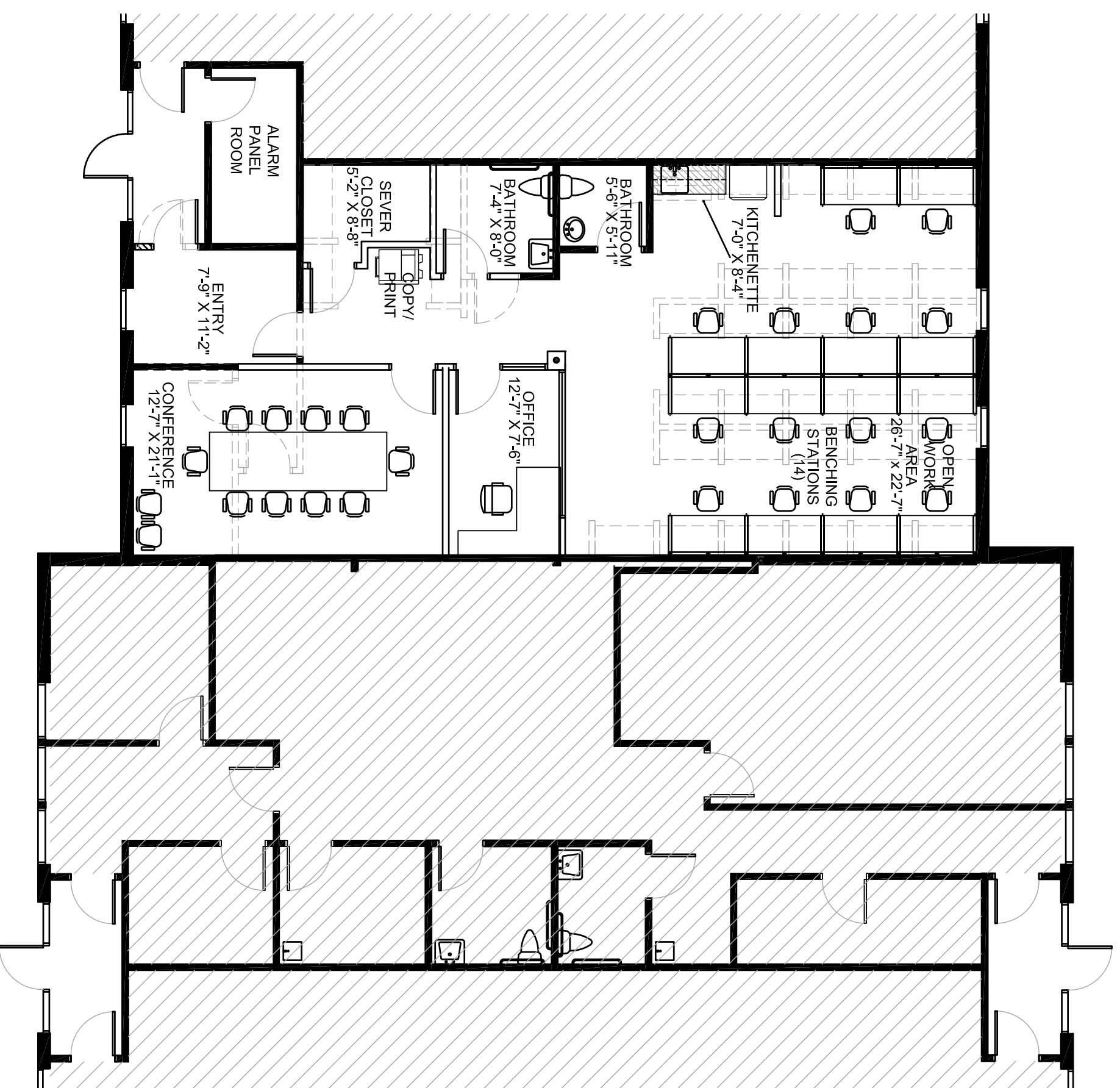
Proposed Space Plan - Ground Floor Scale: 1/8" = 1'-0"
