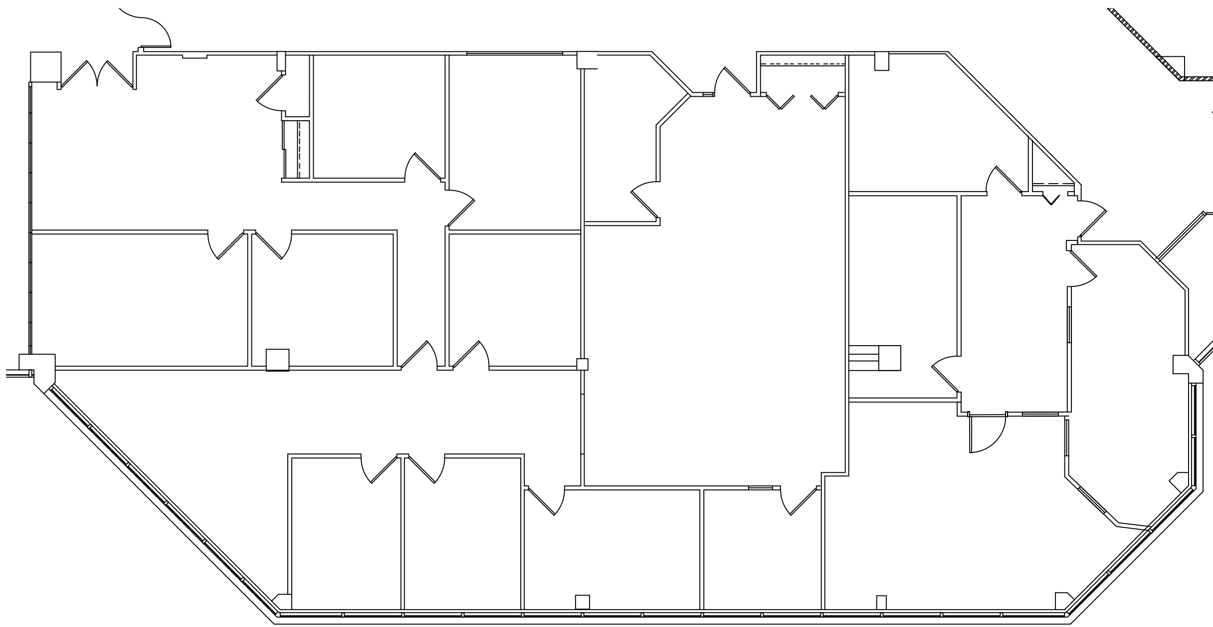
KEY PLAN - FIRST FLOOR SCALE: NOT TO SCALE
